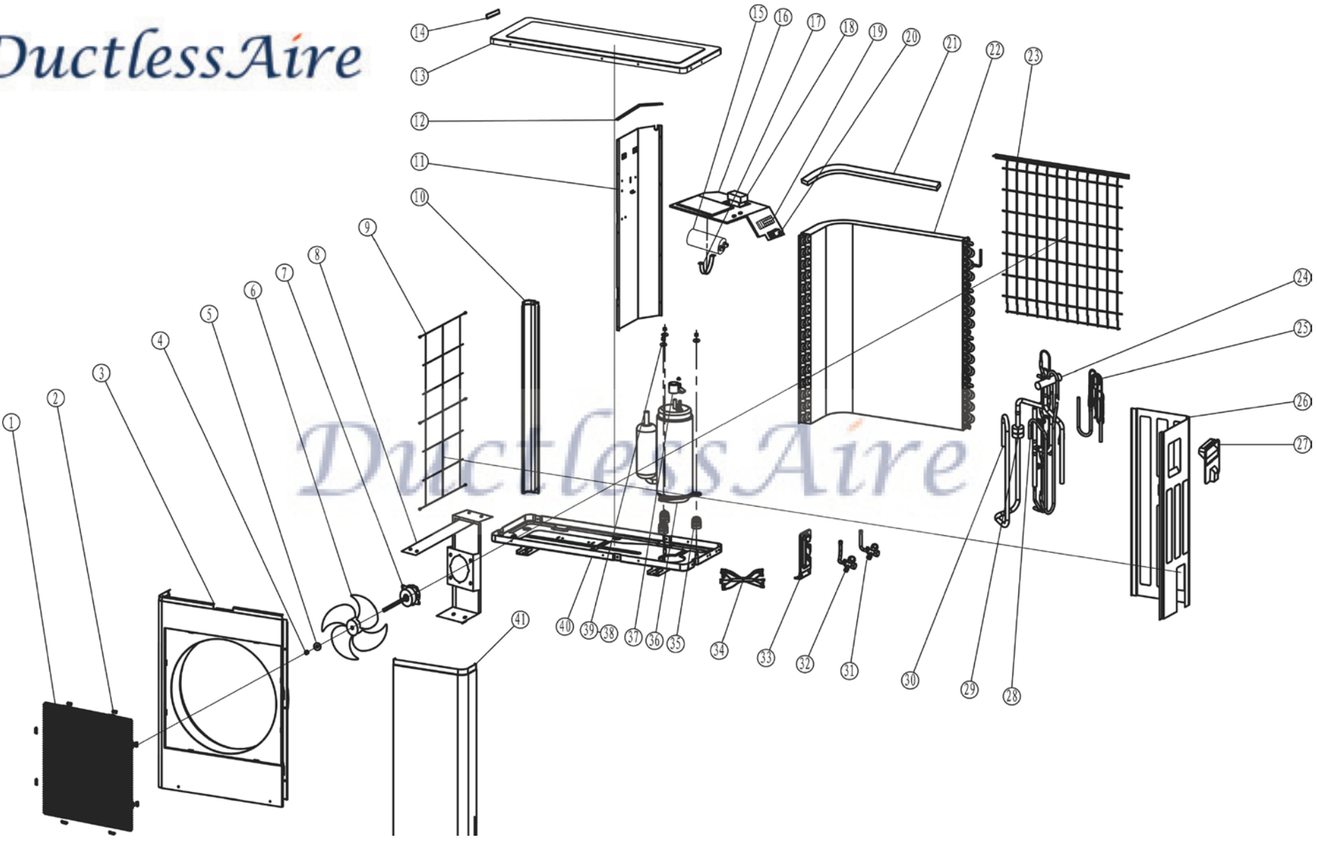
DA2413-H230/O OUTDOOR UNIT EXPLODED VIEW
